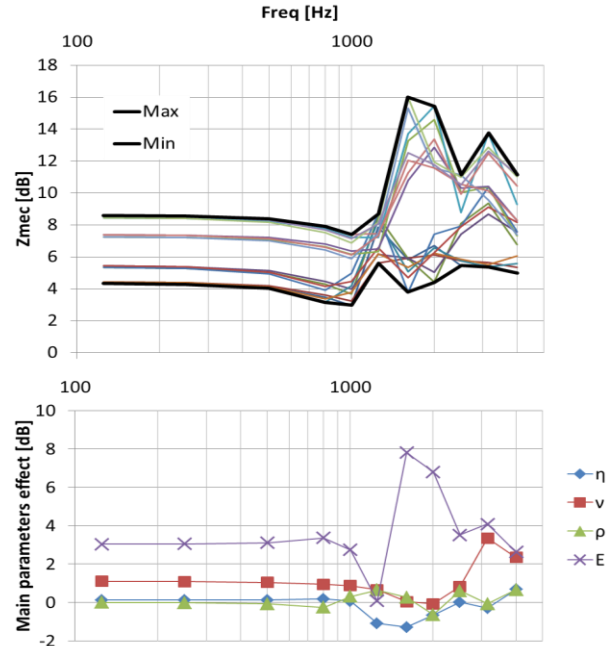
Figure 2: Z_{mec} at position P2 in third octave bands obtained for each combination of parameters (16 runs) (top) and the associated first order effects of the material's properties (bottom).
