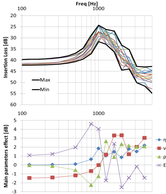
Figure 1: Insertion loss in third octave bands computed for each combination of parameters (16 runs) (top) and the associated first order effects of the material's properties (bottom).
