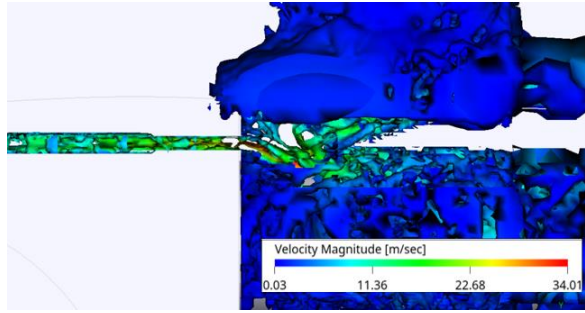
Figure 3: \lambda_2 criterion applied to the recorder.
