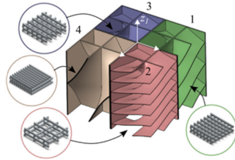
Figure 1. Schematic of parallel assembly of four folded metaporous materials [4].
