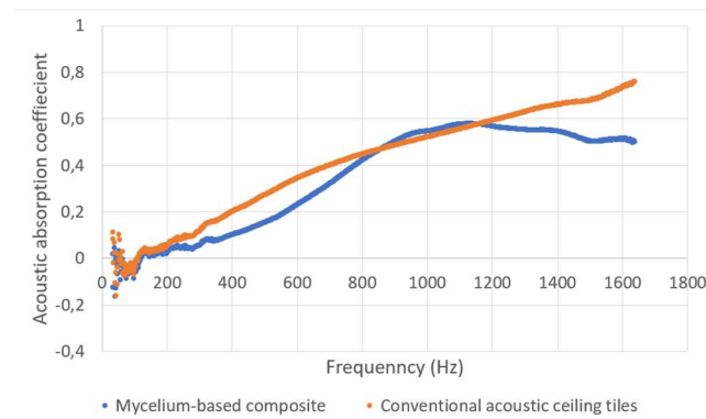
Figure 3: Sound absorption coefficients of mycelium-based composite and conventional acoustic ceiling tiles measured in impedance tube.
