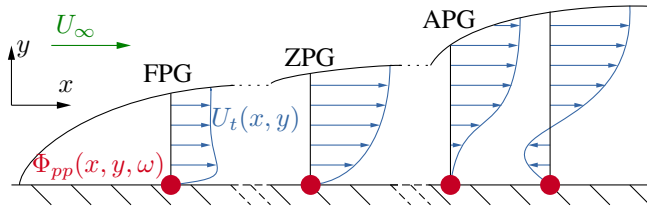
Figure 1: Boundary layer development on a flat plate. Forward, zero and adverse pressure gradient effects.
