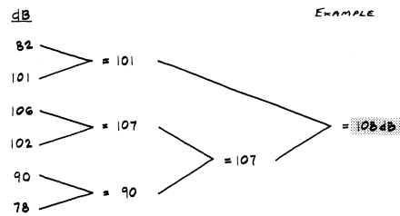
Figure 5: Decibel Addition [1, 2].
